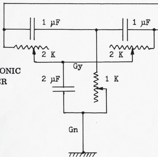
MAGNETIC ANALYSER - POWER SUPPLY, BRIDGE, HARMONIC FILTER, AND RANGE SELECTOR
