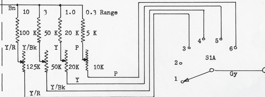
MAGNETIC ANALYSER - POWER SUPPLY, BRIDGE, HARMONIC FILTER, AND RANGE SELECTOR
