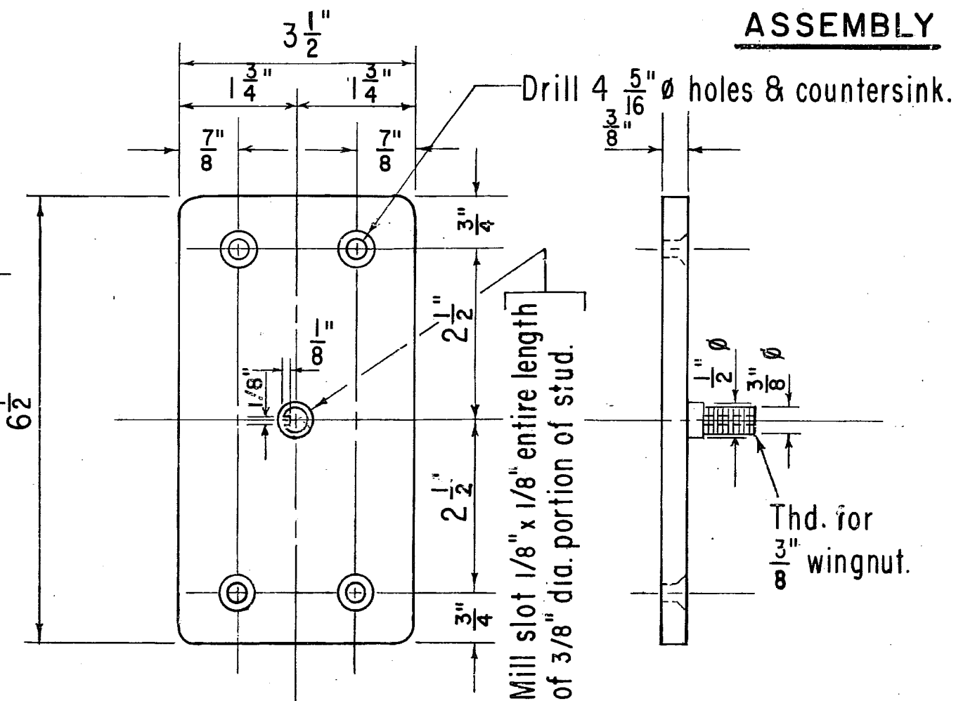
WALL BRACKET
