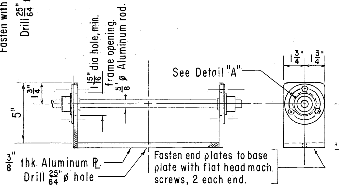
BASE PLATE
