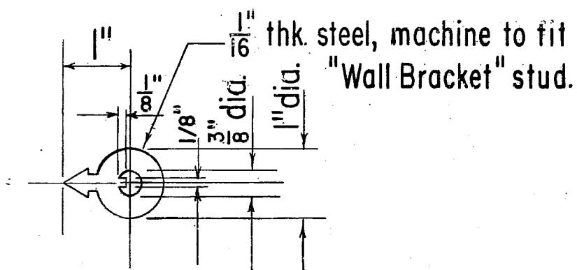
POINTER
