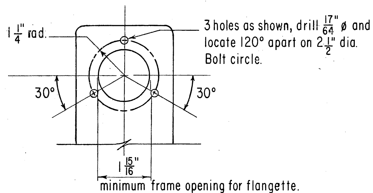
DETAIL "A"
