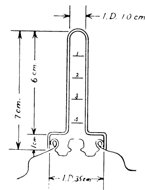
FIG. 2 Suggested Tube for Evaluation of Valve, and Staked and Clinched Seals
