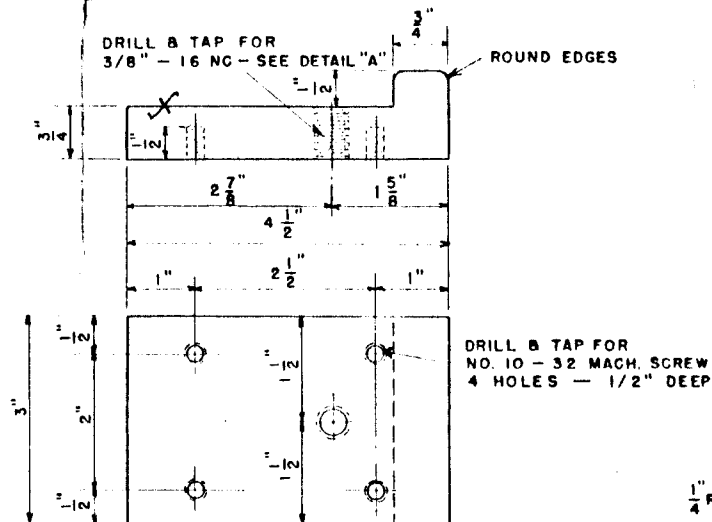
ITEM 2-BOTTOM PLATE-2 REQ'D MATERIAL-COPPER
