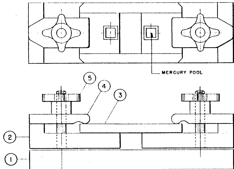
ASSEMBLY
