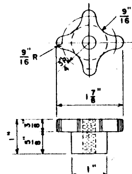
ITEM 5-CLAMPING KNOB-2 REQ'D MATERIAL-STEEL
