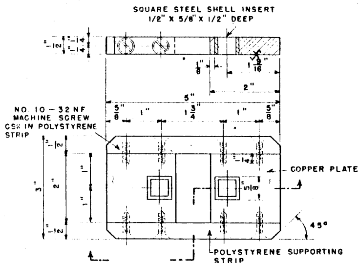
ITEM 3-UPPER PLATE-1 REQ'D MATERIAL-COPPER & POLYSTYRENE
