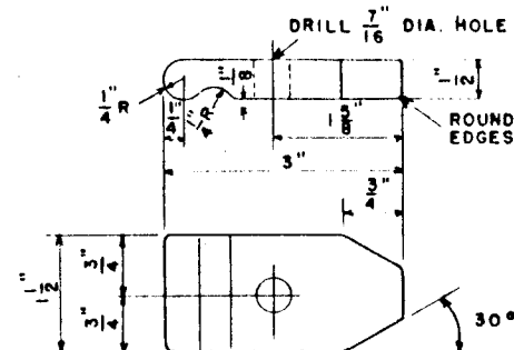
ITEM 4-CLAMP-2 REQ'D MATERIAL-BRONZE
