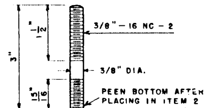
DETAIL "A" - 2 REQ'D MATERIAL-STEEL
