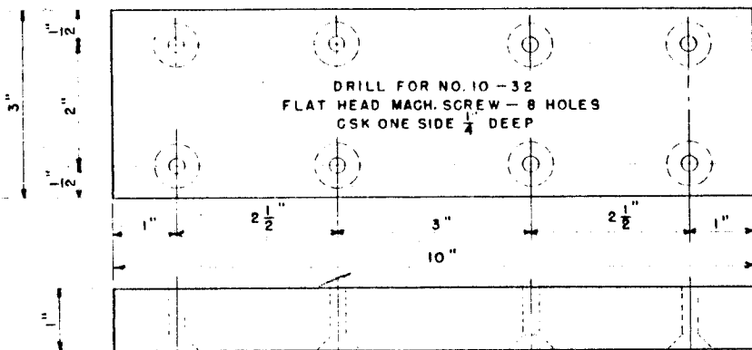
ITEM 1-BASE-1 REQ'D MATERIAL-POLYSTYRENE
