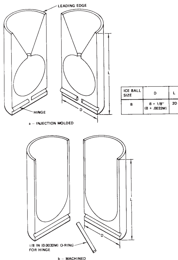
FIG. 1 Sabot Configuration
