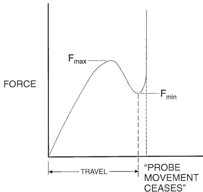
FIG. 1 Typical Tactile Force—Travel Curve
